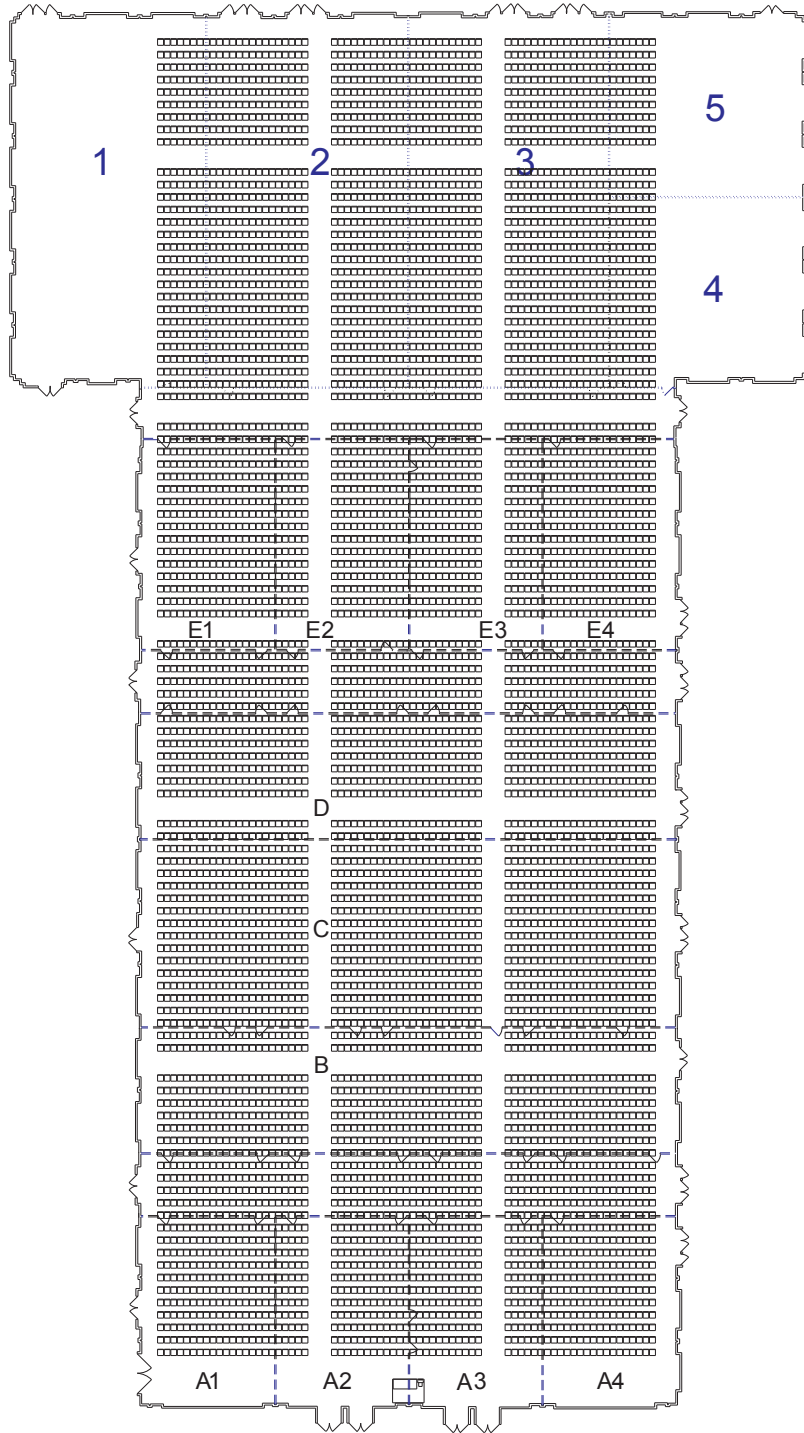
WALT DISNEY WORLD DOLPHIN HEMISPHERES BALLROOM AREA 54,238 SQ. FT. CEILING 27 FT. 4 IN. LOWEST PT. 22 FT. 2 IN. Theater 0 32 64 1/64" = 1' 6,457 Chairs
