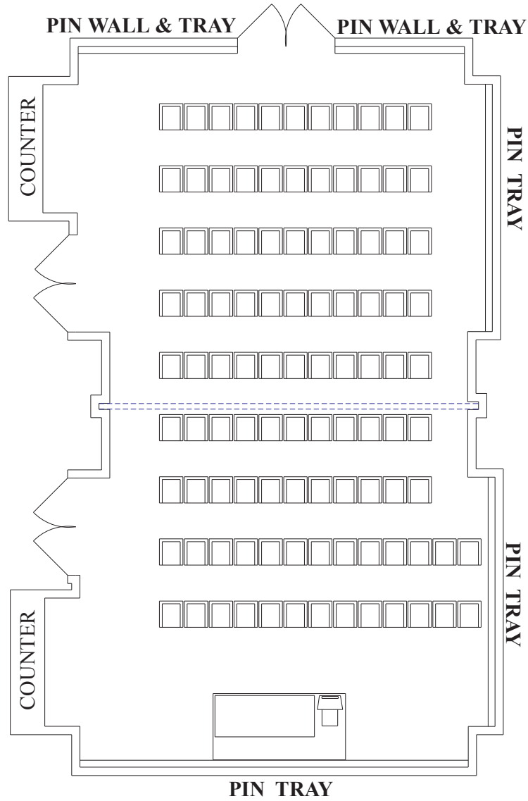
WALT DISNEY WORLD SWAN LARK AREA 1,085 SQ. FT. CEILING 12 FT. 2 IN. LOWEST PT. 10 FT. 10 IN. Theater 0 4 8 103 Chairs 1/8" = 1'
