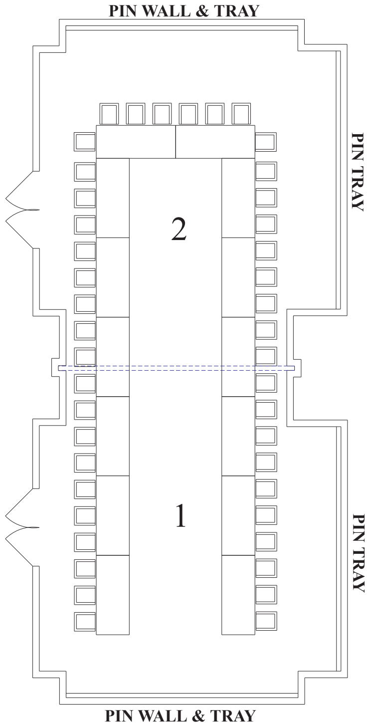
WALT DISNEY WORLD SWAN PARROT AREA 1,248 SQ. FT. CEILING 13 FT. 0 IN. LOWEST PT. 13 FT. 0 IN. U-shape 0 4 8 1/8" = 1' 47 Chairs
