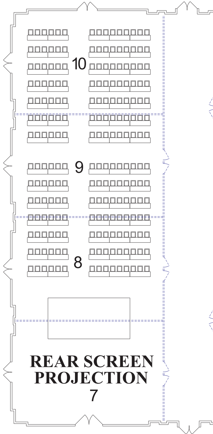
WALT DISNEY WORLD SWAN SWAN 7-10 REAR SCREEN PROJECTION AREA 5,291 SQ. FT. CEILING 23 FT. 6 IN. LOWEST PT. 22 FT. 7 IN. Schoolroom 0 8 16 1/16" = 1' 210 Chairs
