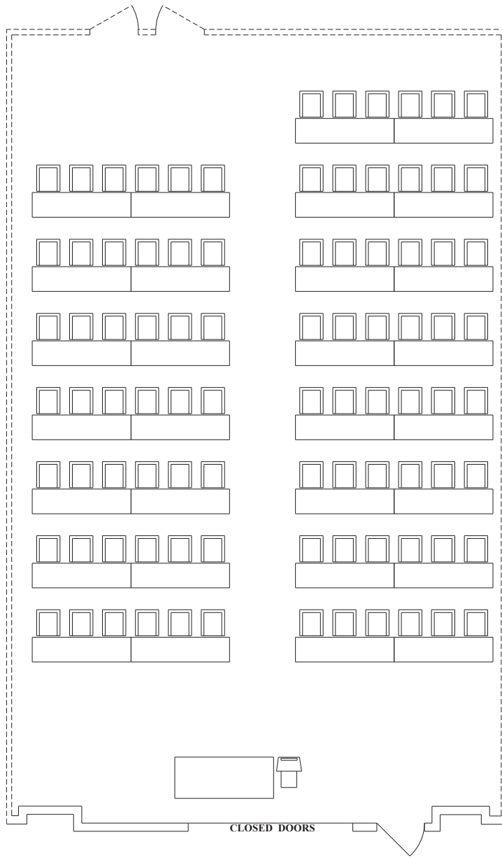
WALT DISNEY WORLD SWAN SWAN 3 AREA 1,416 SQ. FT. CEILING 22 FT. 0 IN. LOWEST PT. 22 FT. 0 IN. Schoolroom 0 4 8 1/8" = 1' 90 Chairs
