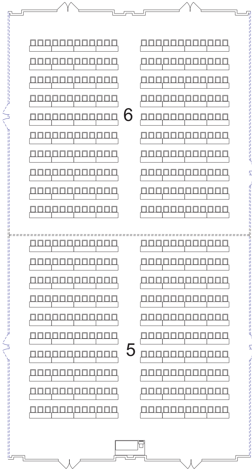
WALT DISNEY WORLD SWAN SWAN 5 & 6 AREA 7,824 SQ. FT. CEILING 23 FT. 6 IN. LOWEST PT. 22 FT. 7 IN. Schoolroom 0 8 16 480 Chairs 1/16" = 1'
