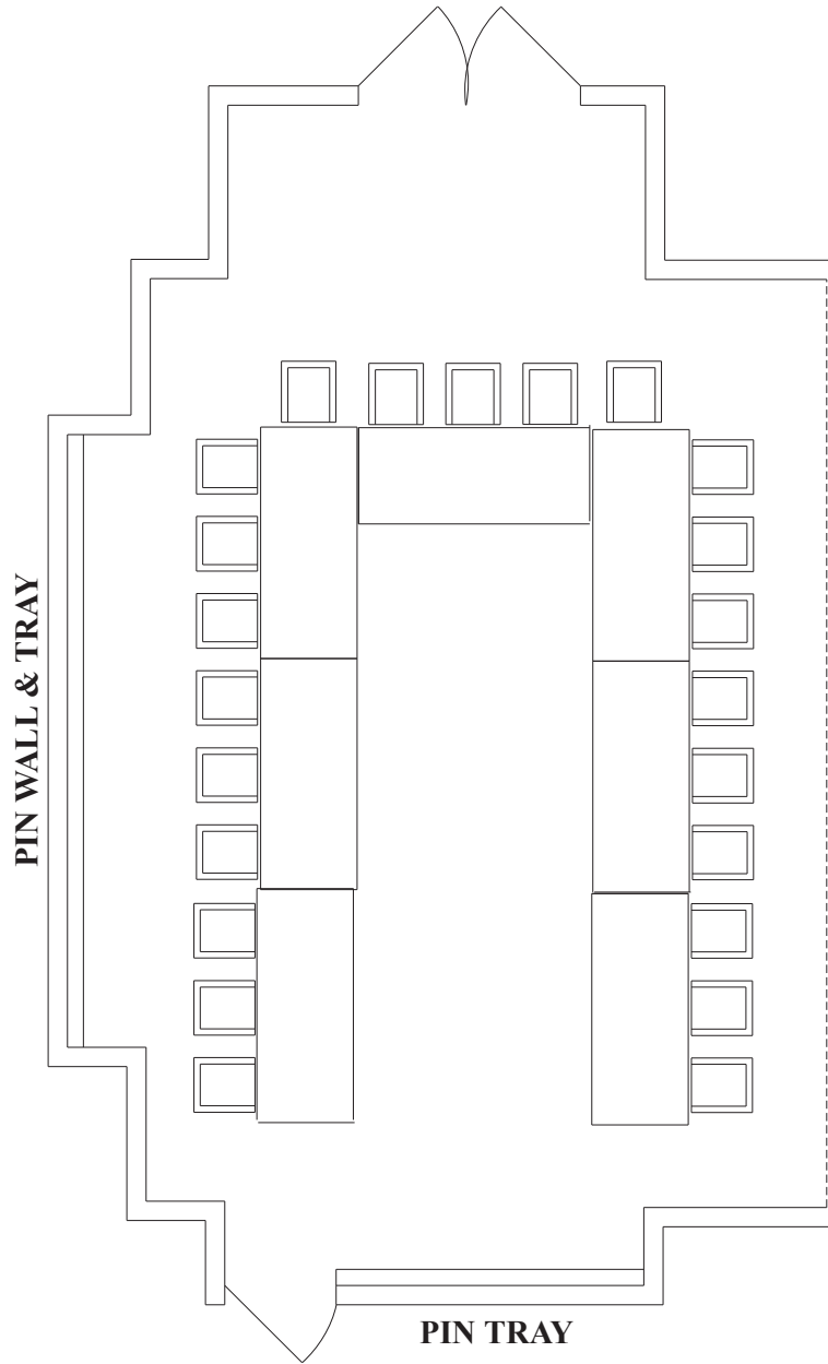
WALT DISNEY WORLD SWAN TOUCAN 1 AREA 530 SQ. FT. CEILING 12 FT. 2 IN. LOWEST PT. 10 FT. 10 IN. U-shape 0 2 5 3/16" = 1' 23 Chairs
